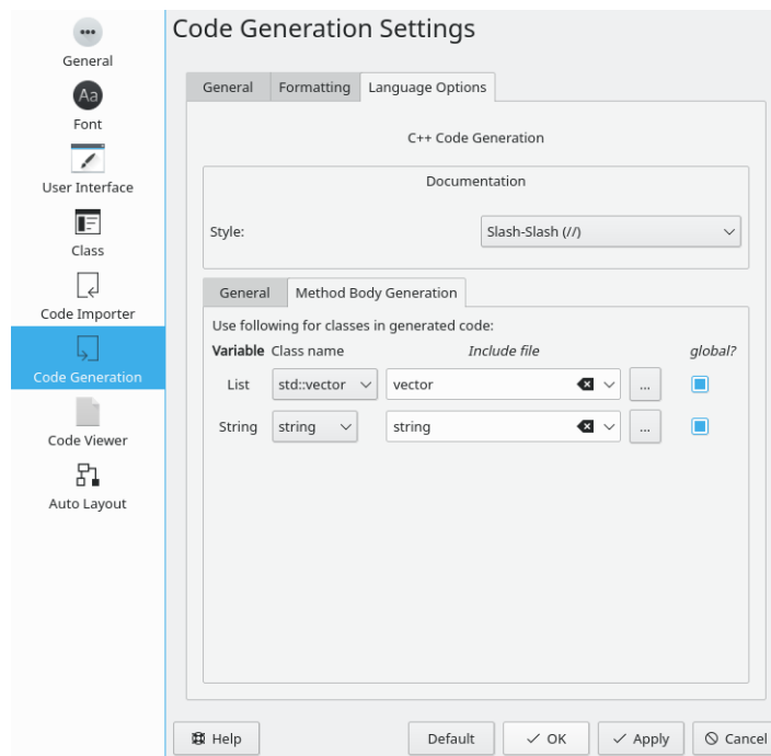
Options for the Code Generation Language Method Body Settings in Umbrello UML Modeller
